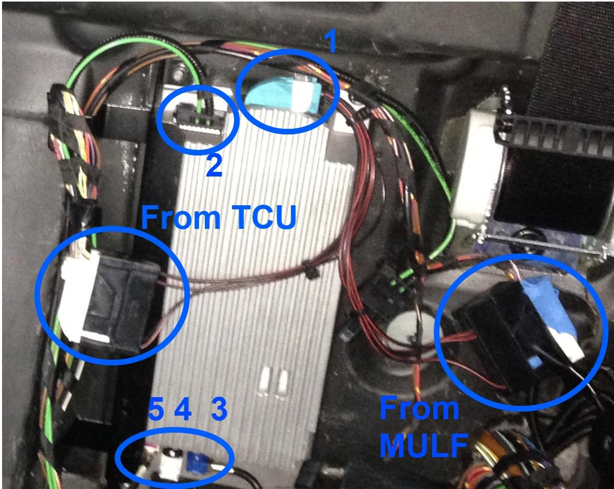
Figure 22 Combox installed
