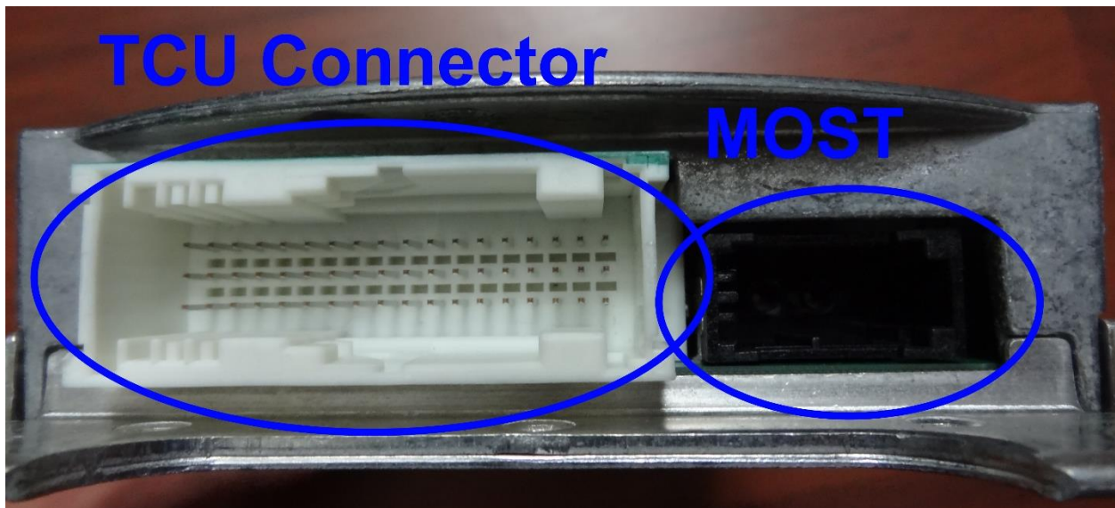
Figure 21 TCU connections
