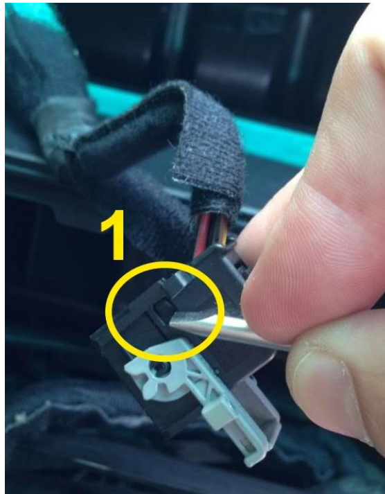
Figure 9 CCC Display Connector Tab
