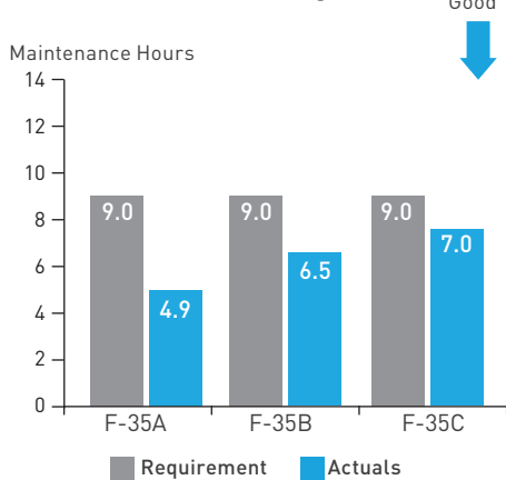
Maintainability: Maintenance Man Hour Per Flight Hour
