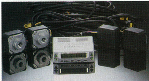
TEIN's EDFC system includes four stepper motors mounted on top of each shock tower and an electronic control unit.
